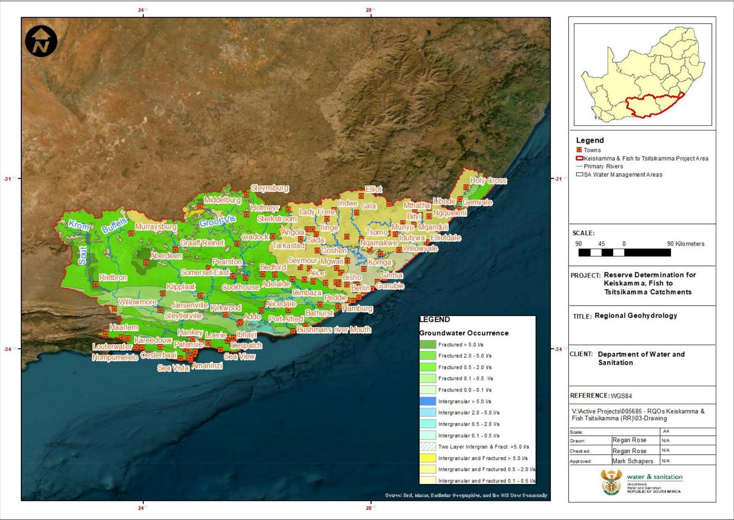
Figure 2: Regional Geohydrology
