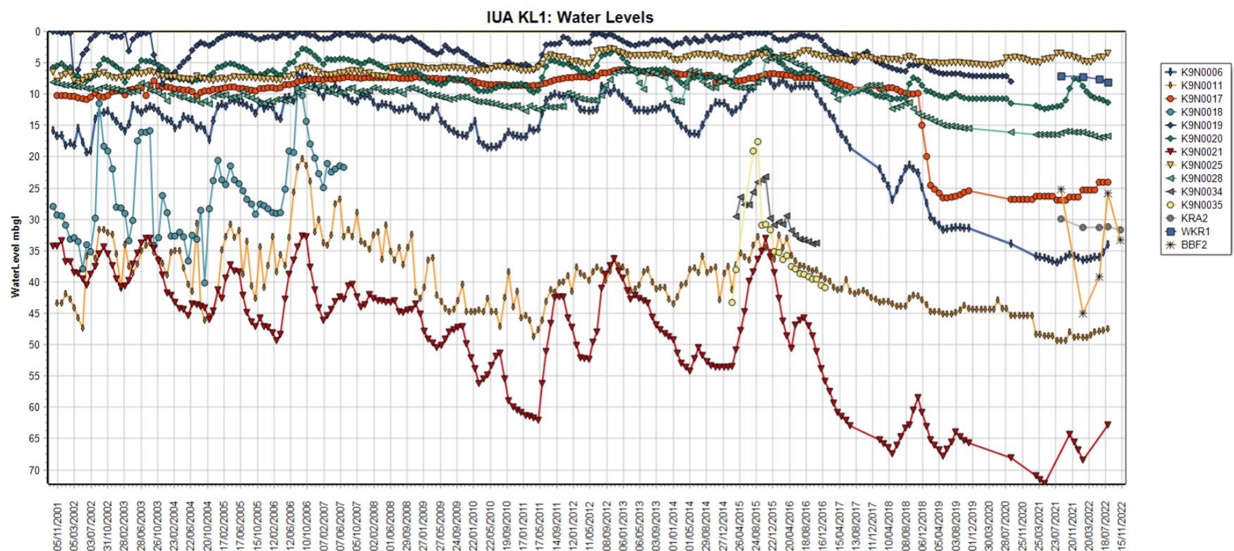
Figure 14: IUA KL1 Water Levels
