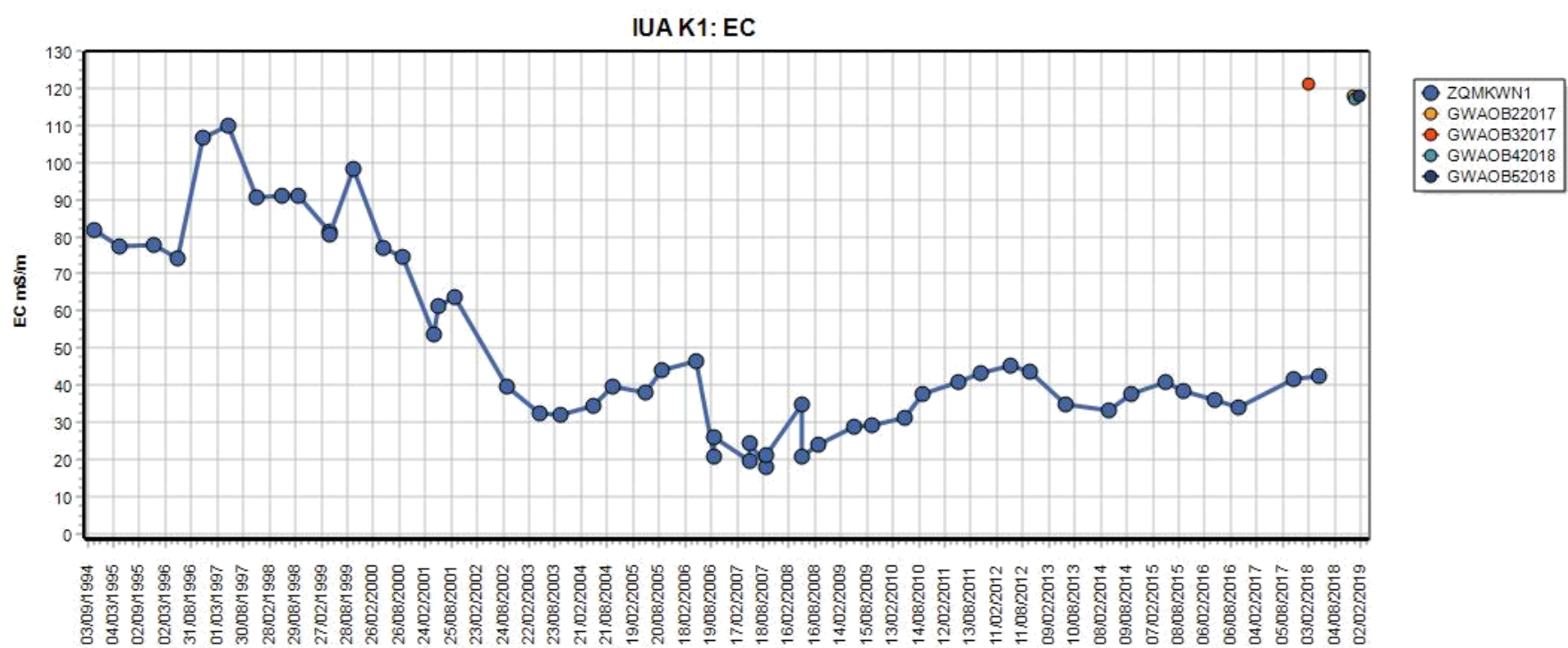
Figure 13: IUA K1 EC
