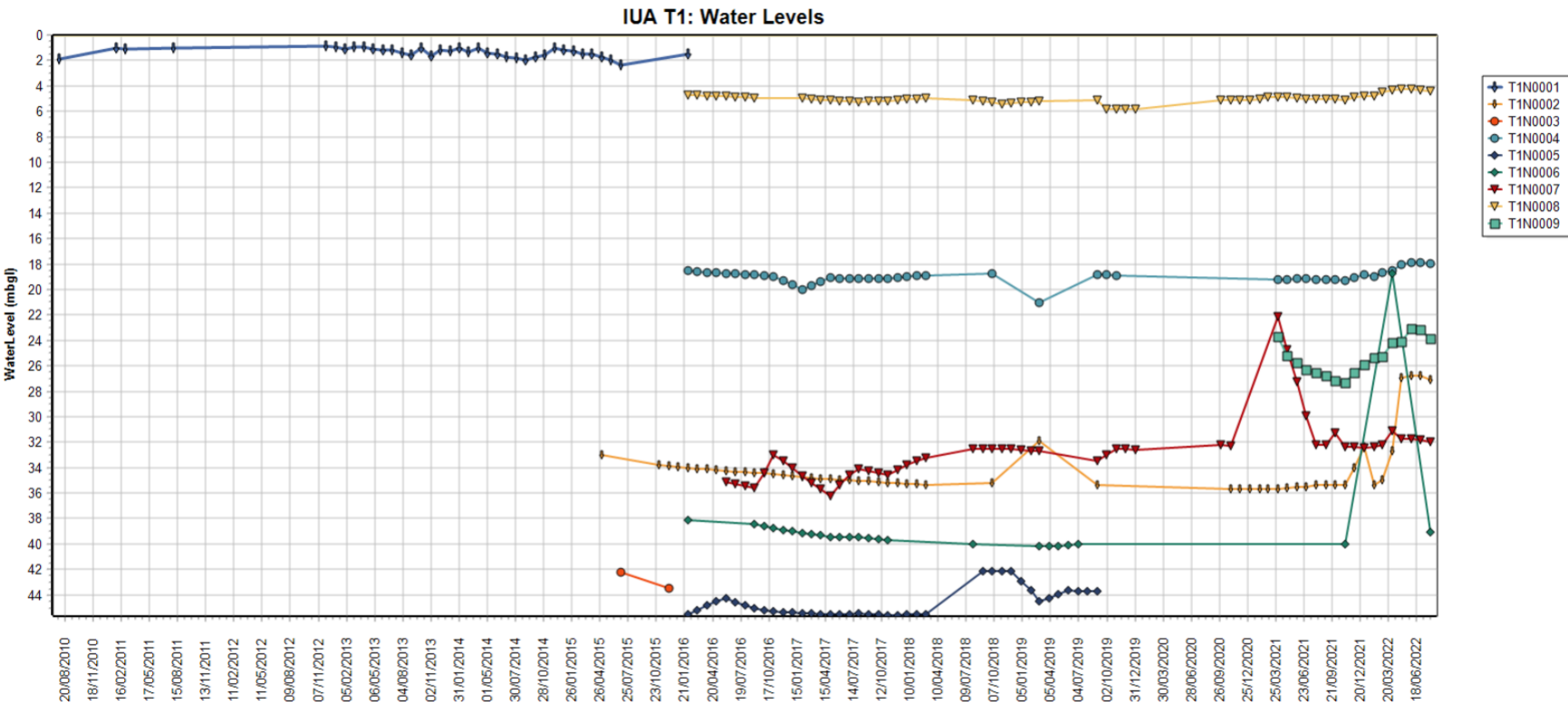
Figure 38: IUA T1 Water Levels
