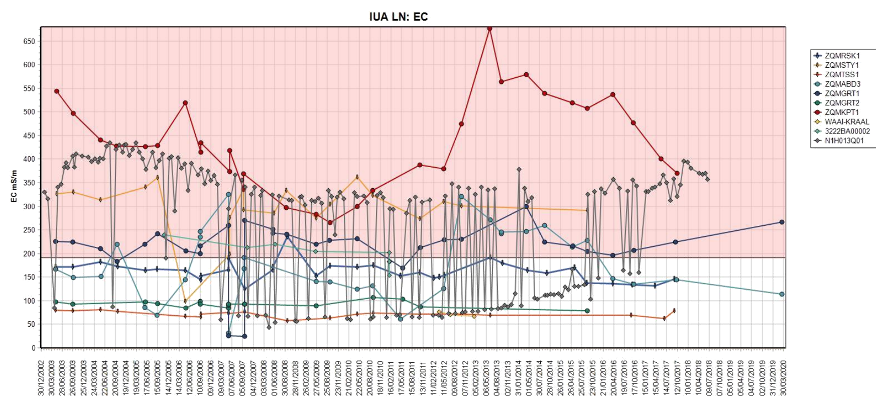
Figure 19: IUA LN1 EC
