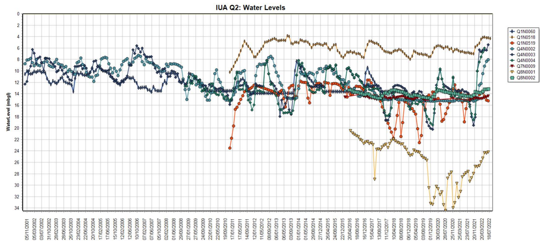
Figure 27: IUA Q2 Water Levels
