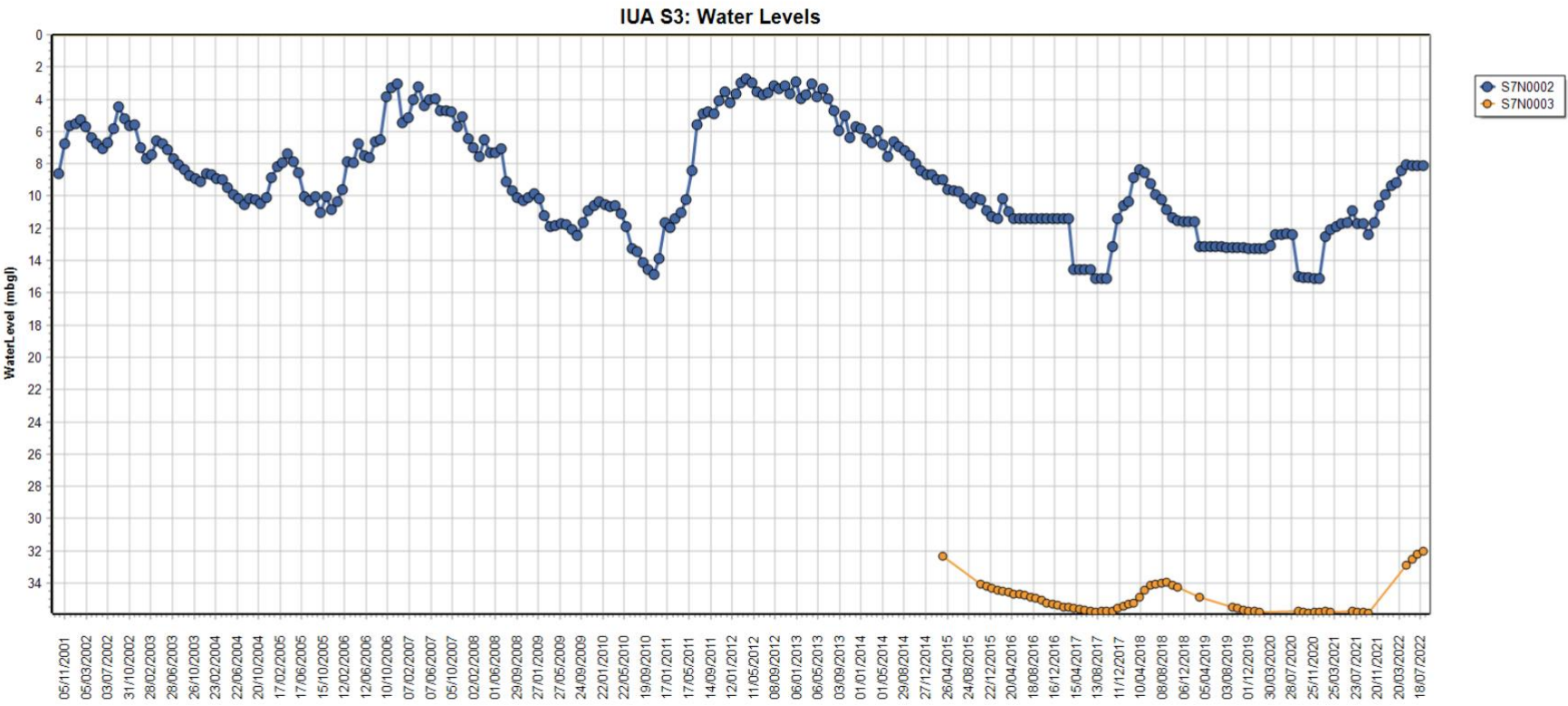
Figure 36: IUA S3 Water Levels
