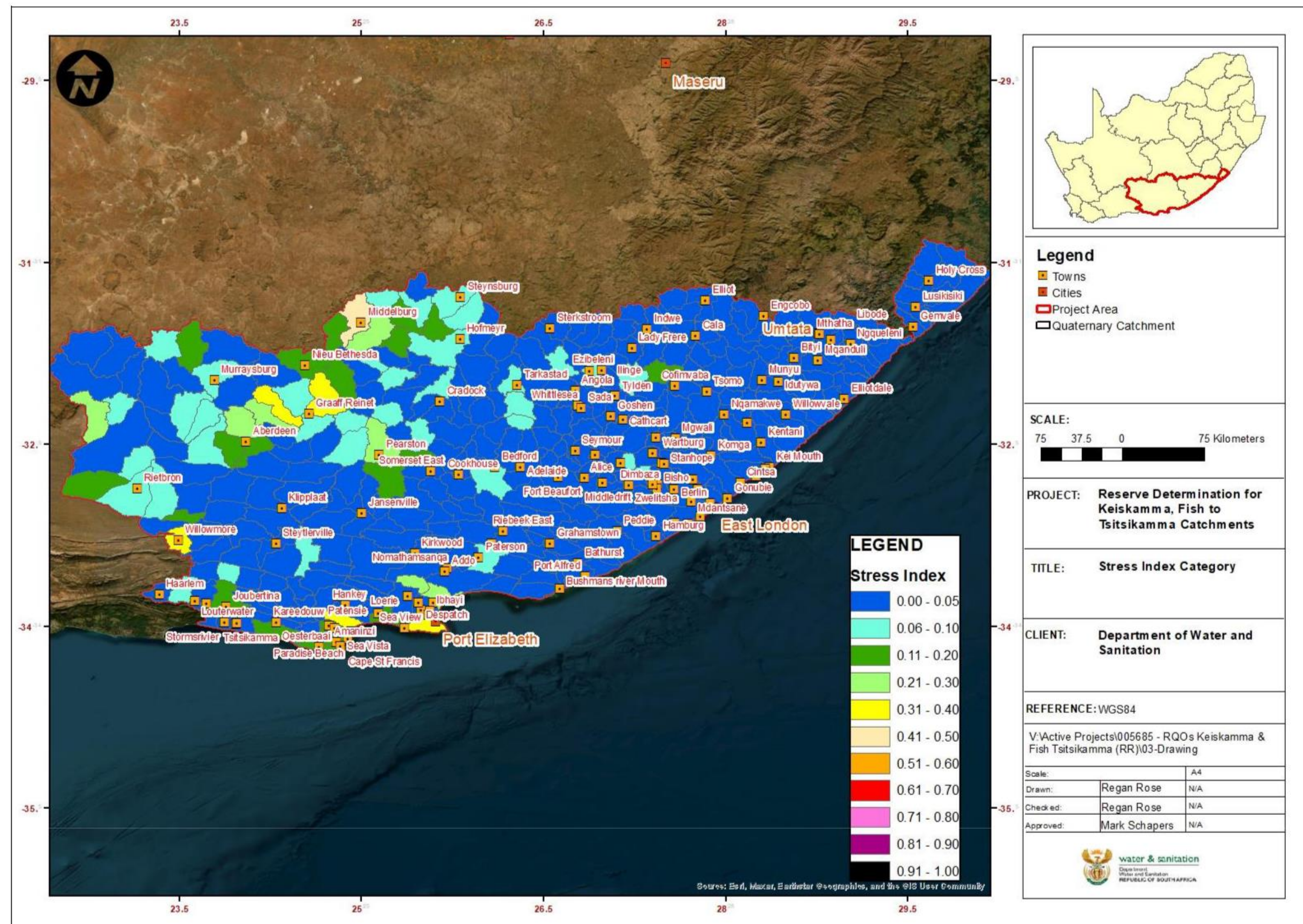
Figure 10: Stress Index distribution in the catchment
