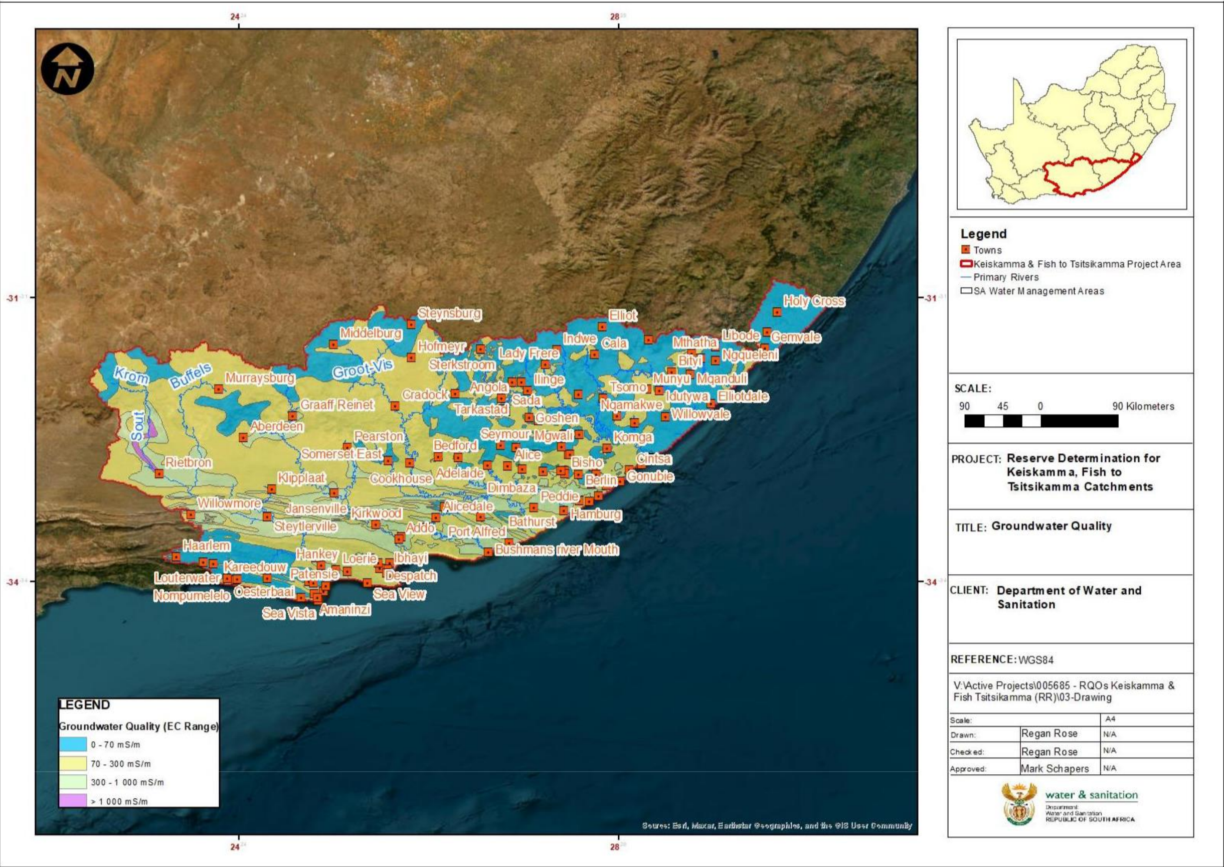
Figure 3: Regional Groundwater Quality
