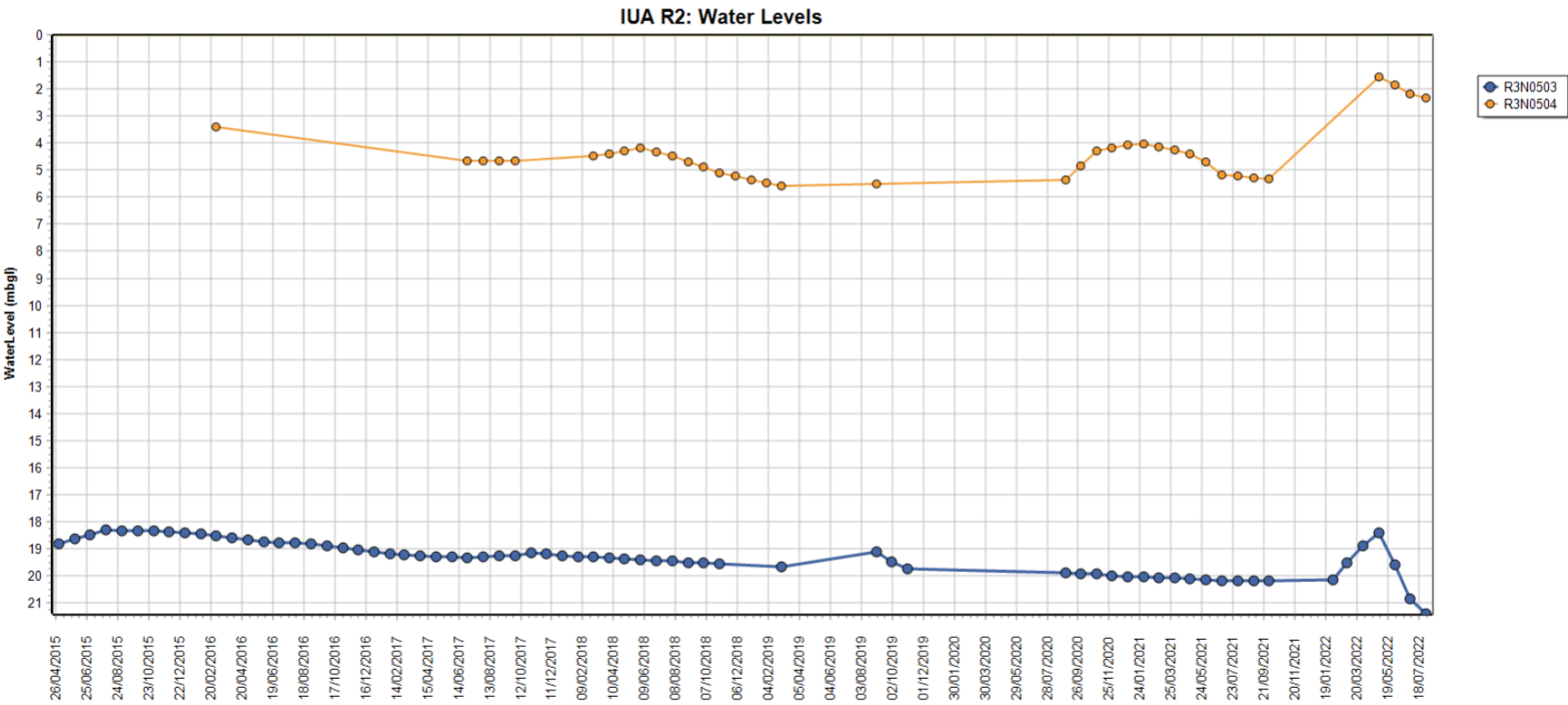
Figure 30: IUA R2 Water Levels
