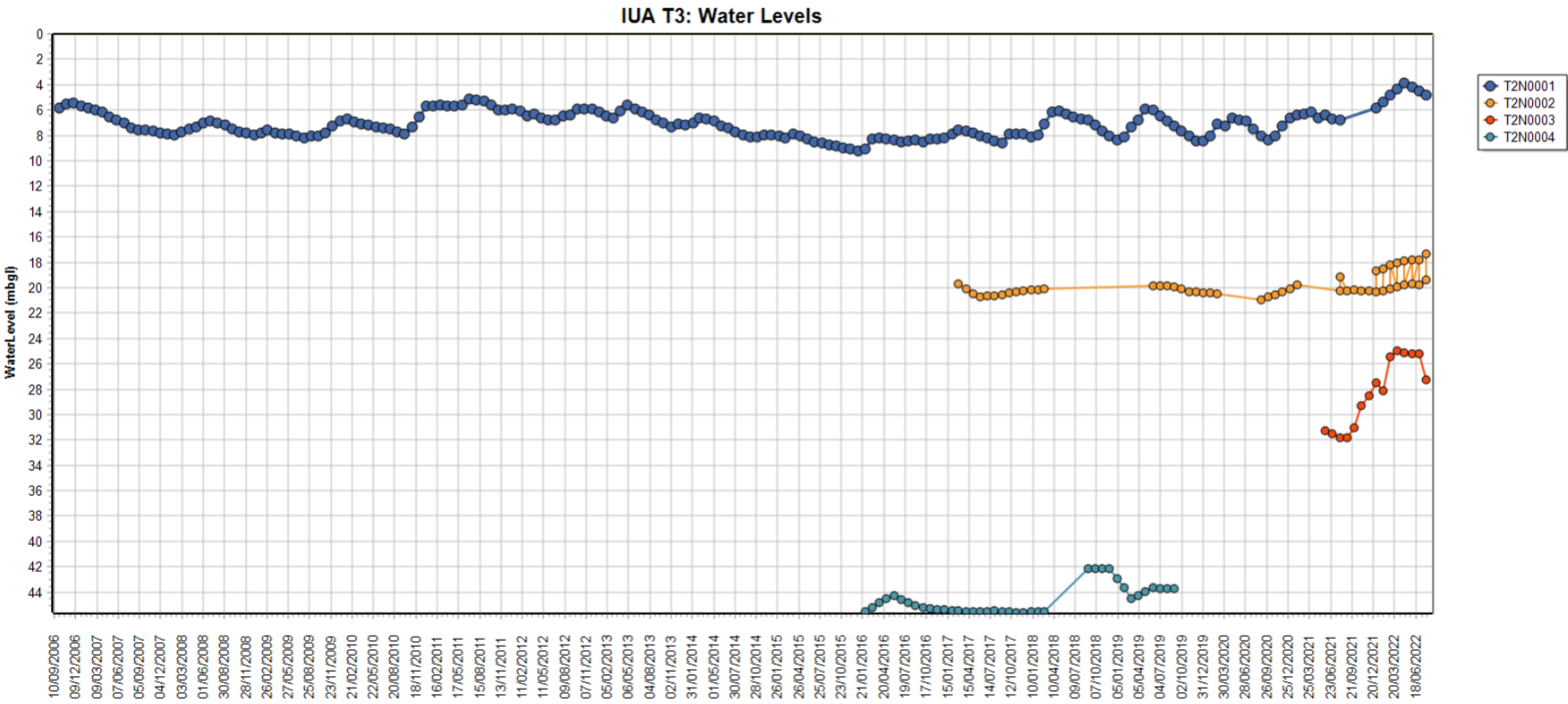
Figure 41: IUA T3 Water Levels
