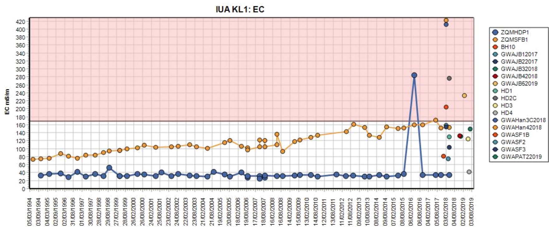
Figure 15: IUA KL1 EC
