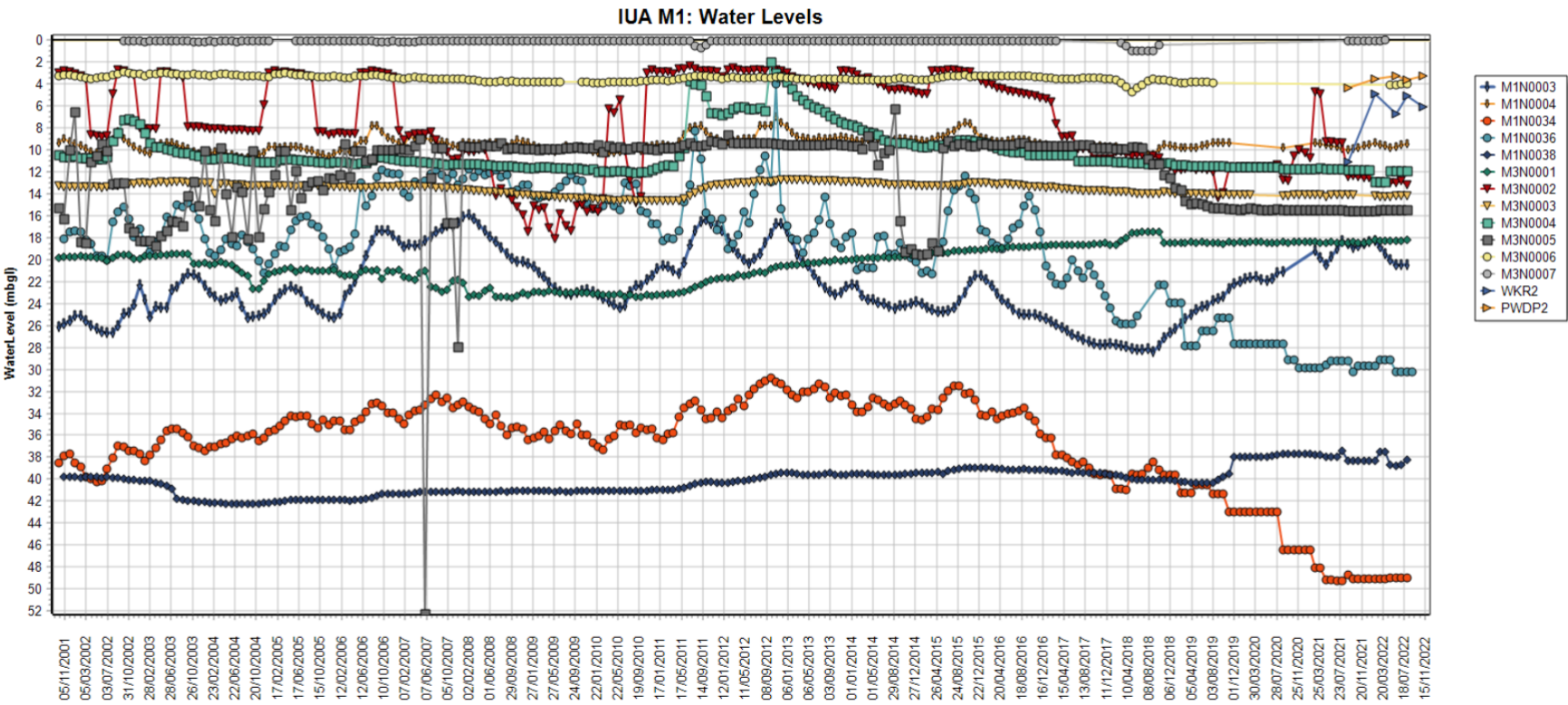
Figure 20: IUA M1 Water Levels
