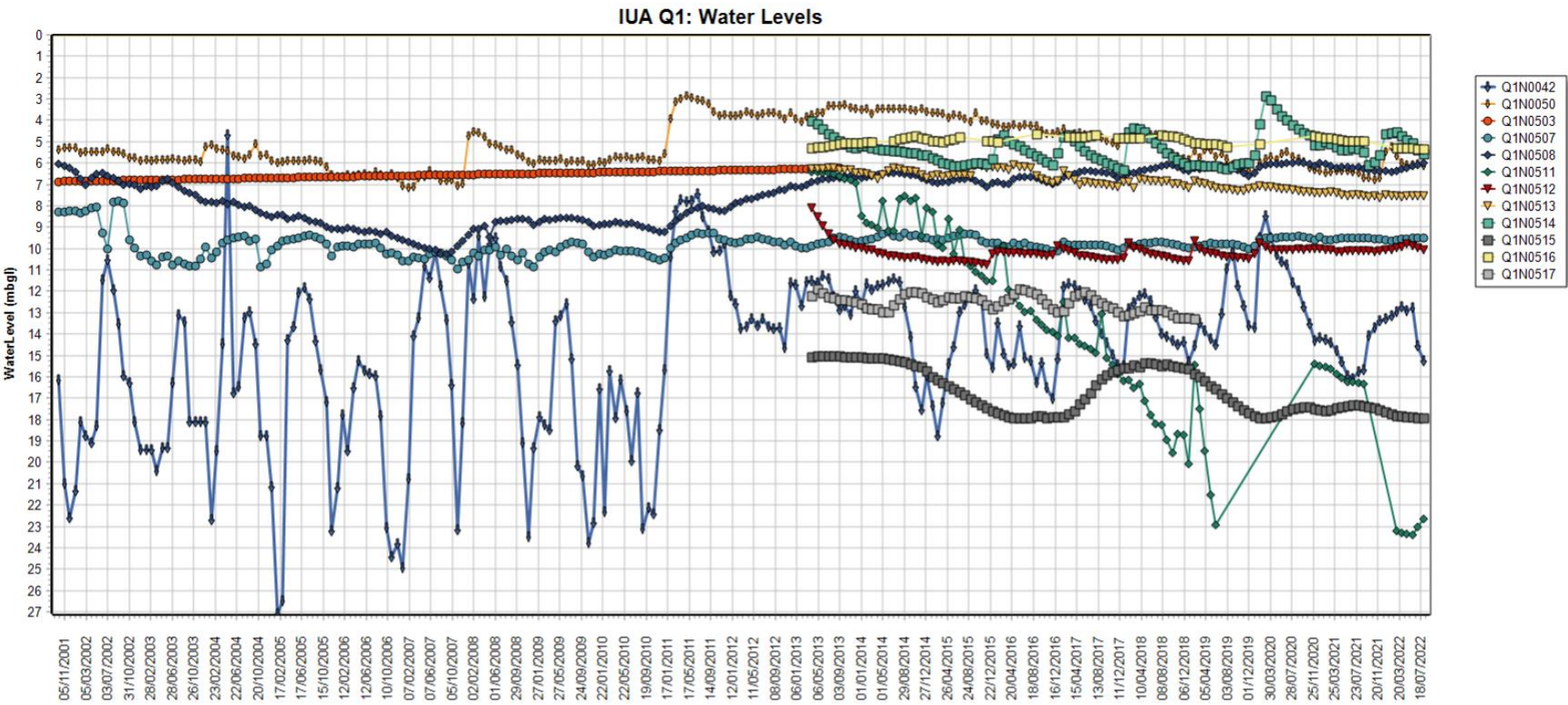
Figure 25: IUA Q1 Water Levels
