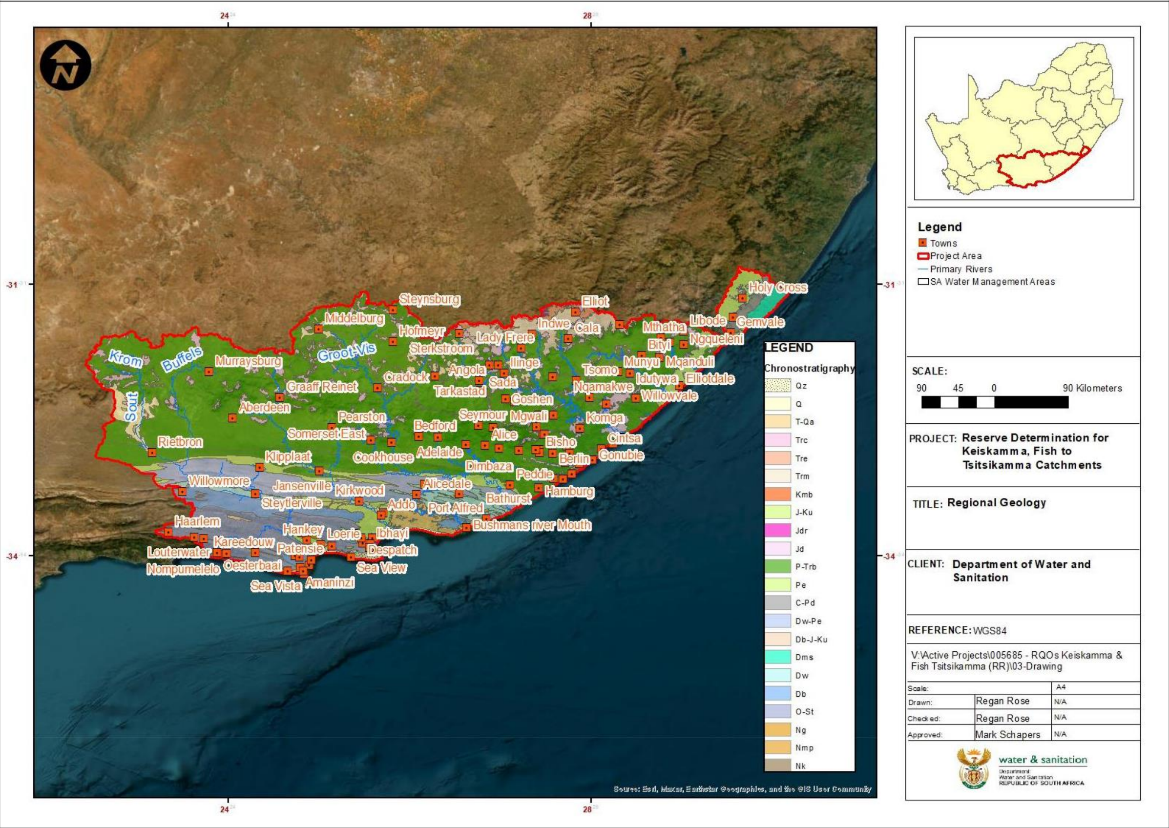
Figure 1: Regional Geology
