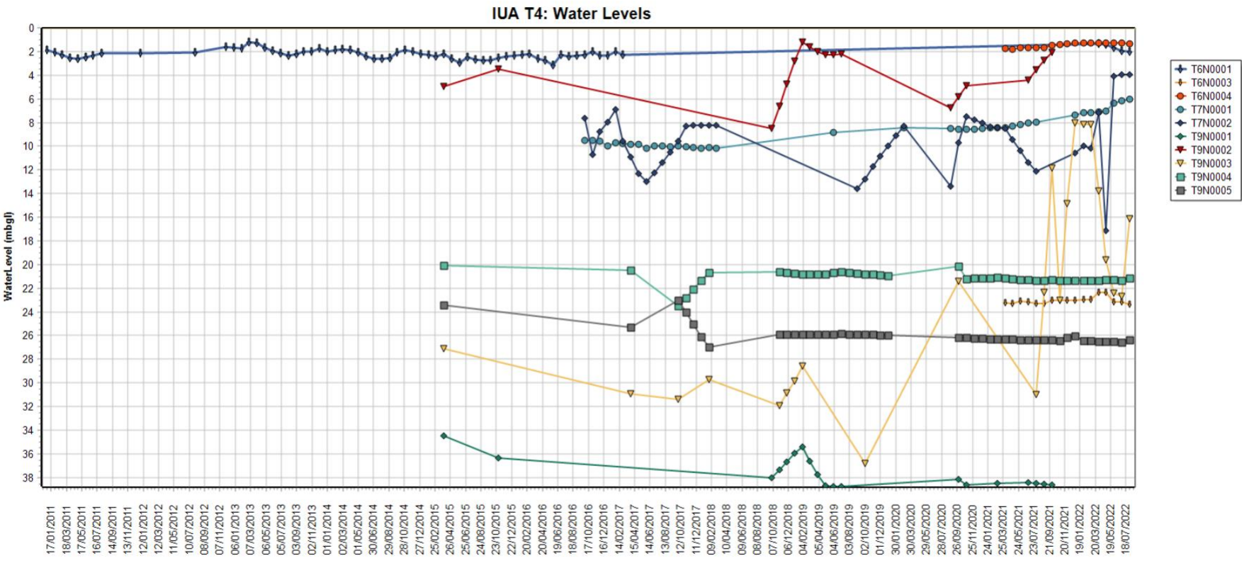
Figure 43: IUA T4 Water Levels
