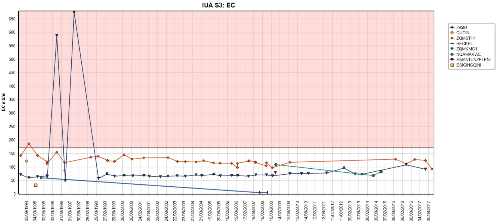
Figure 37: IUA S3 EC
