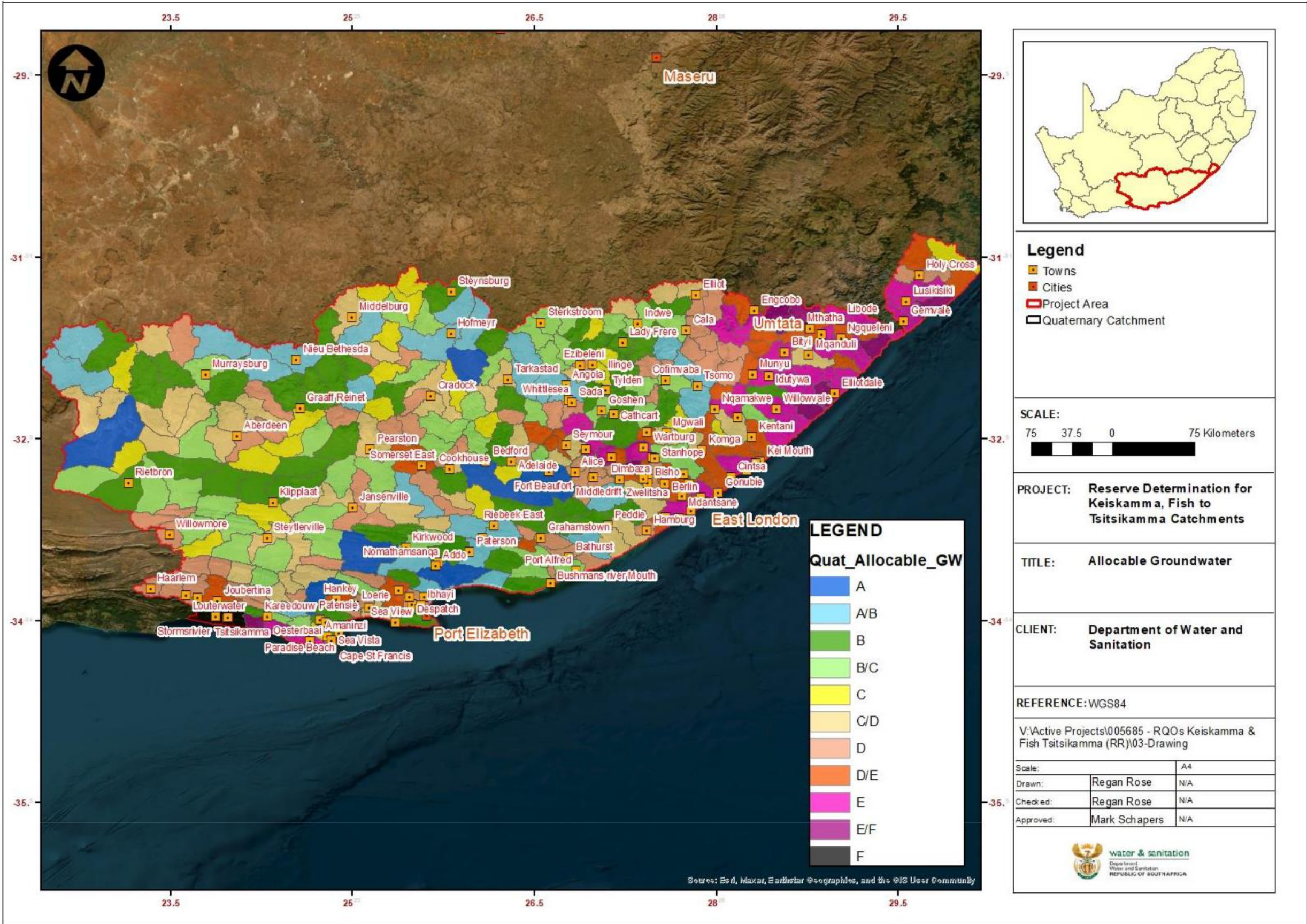
Figure 11: Allocable Groundwater distribution in the catchment
