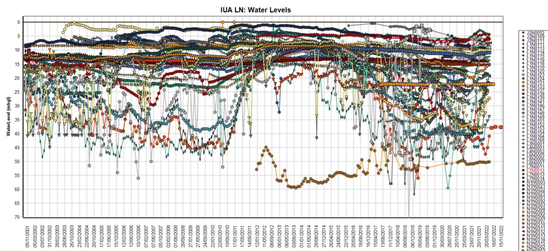
Figure 18: IUA LN1 Water Levels
