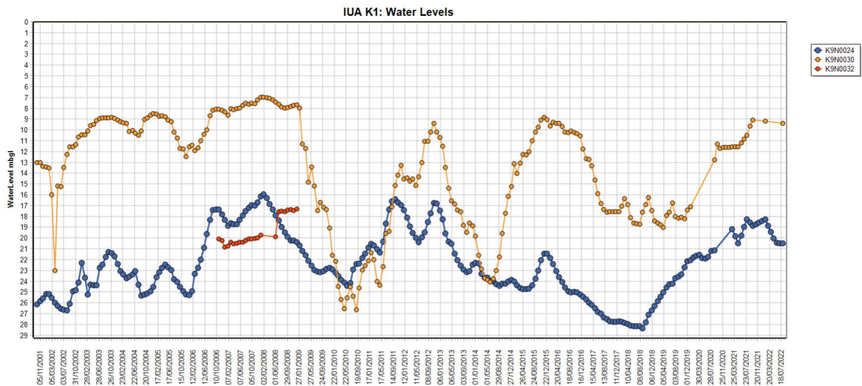
Figure 12: IUA K1 Water Levels
